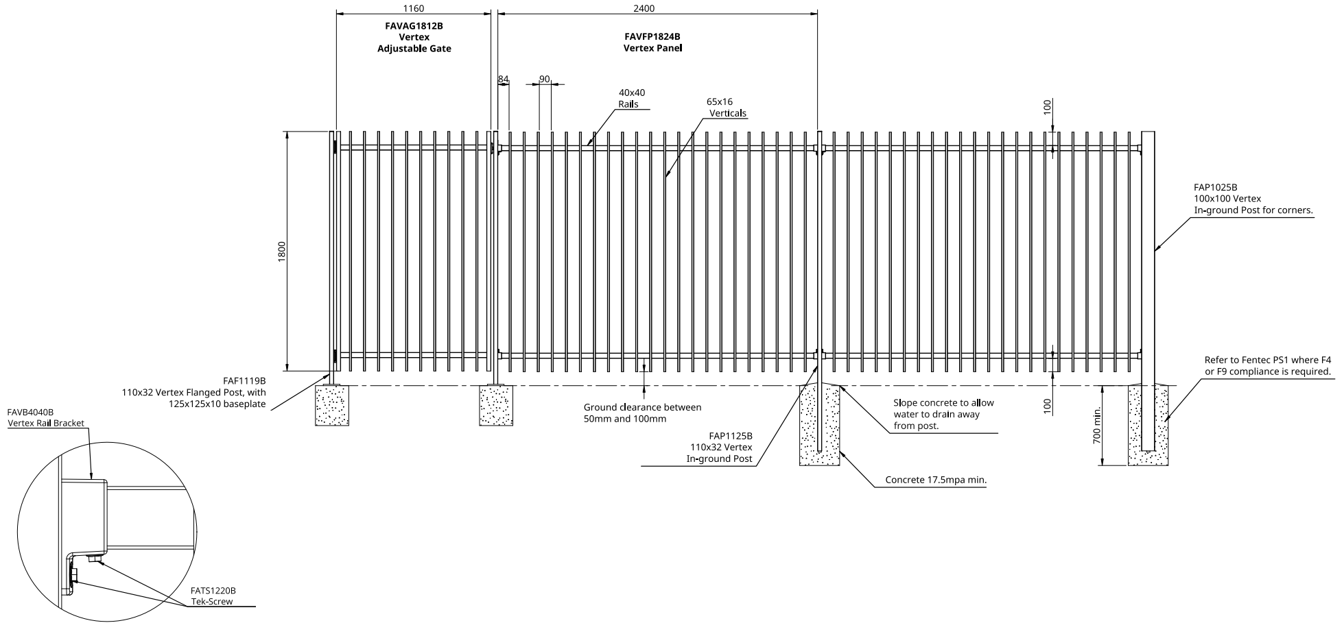
Panel Bracket Detail 1:2
