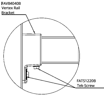
Panel Bracket Detail 1:2
